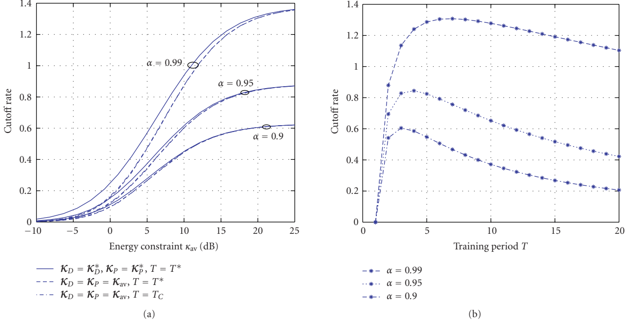
FIGURE 3: The QPSK ( M = 4 ) cutoff rate under the (1,0) estimator for Doppler values \alpha = \{0.90, 0.95, 0.99\} . (a) For fixed \alpha , the solid line represents optimization over the energy allocation and training period \kappa_P = \kappa_P^*, \kappa_D = \kappa_D^* , and T = T^* , the dashed line represents optimization over the training period, but not the energy allocation, \kappa_D = \kappa_P = \kappa_{av} and T = T^* , and the dashed-dotted line represents the unoptimized case, \kappa_D = \kappa_P = \kappa_{av} , and T = T_C (the training period is fixed at the high SNR value determined from (45)). (b) The effect of a suboptimal assignment of the training period T on cutoff rate under the constant energy allocation, \kappa_D = \kappa_P = \kappa_{av} = 20 dB.
