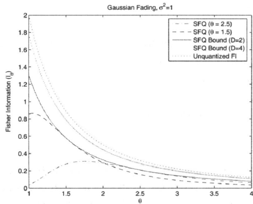
Fig. 4. Gaussian Fading Example
